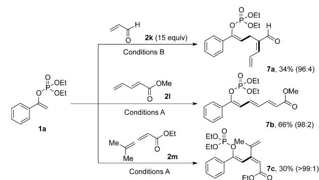
Scheme 2. Synthetic applicability of enol phosphate.
