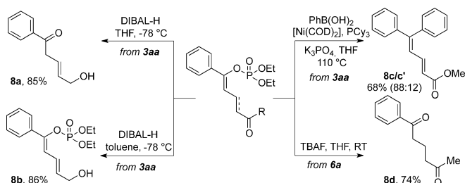
Scheme 3. Synthetic application of the coupling adducts. Dibal-H = diisobutylaluminum hydride, TBAF = tetra- n -butylammonium fluoride, COD = 1,5-cyclooctadiene.
